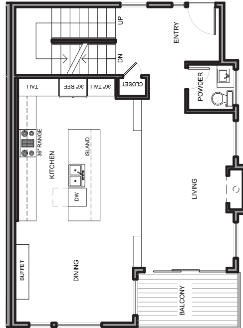
Level 2
