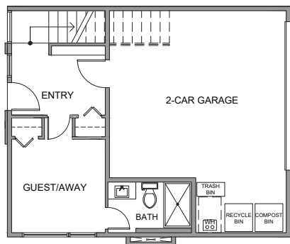
Level 1
