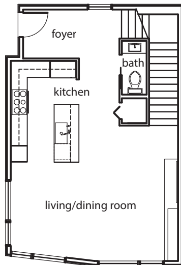
Level 2
