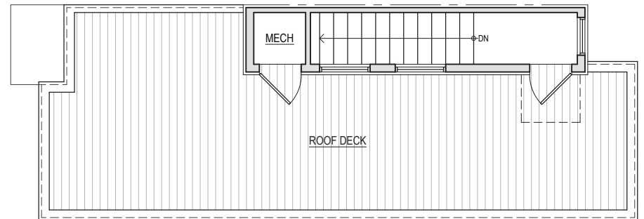
Rooftop
