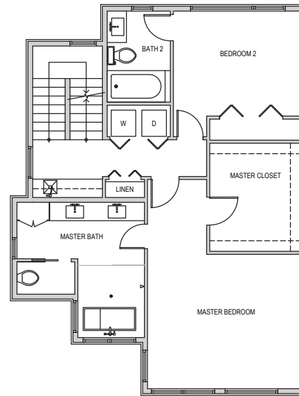
Level 3
