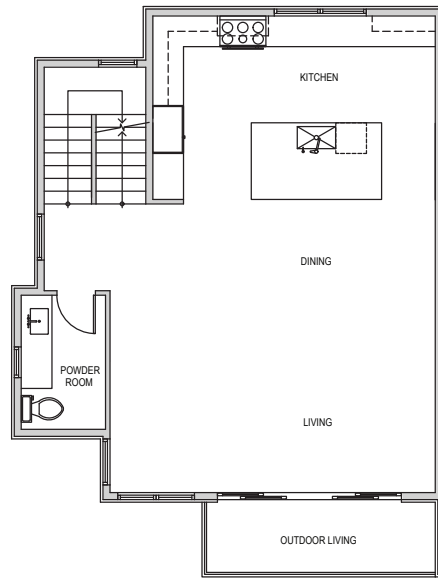
Level 2
