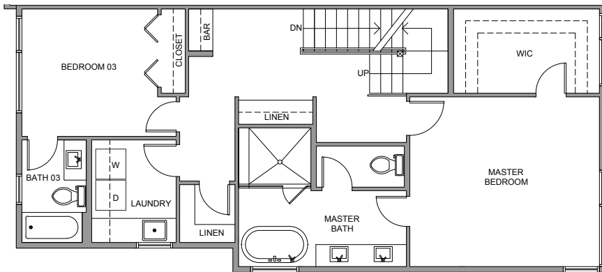
Level 3
