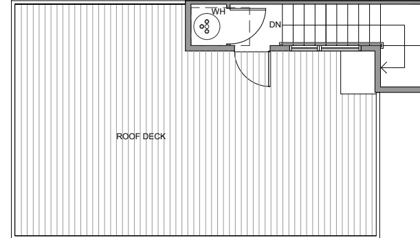
Roof Deck
