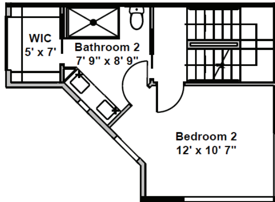
LEVEL 3
