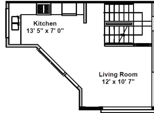
LEVEL 2
